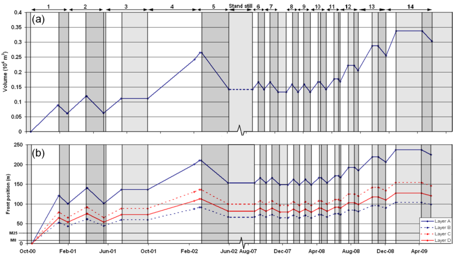
Figure 2.3 (a) Cumulative volume during ASR cycles, (b) Calculated front position of injected water bubble in layers A-D (m distance from ASR well) during both pilots. Effects of bubble drift are not included. Position of monitor wells M8 and M25 indicated (white = injection, light grey = storage, dark grey = recovery).
