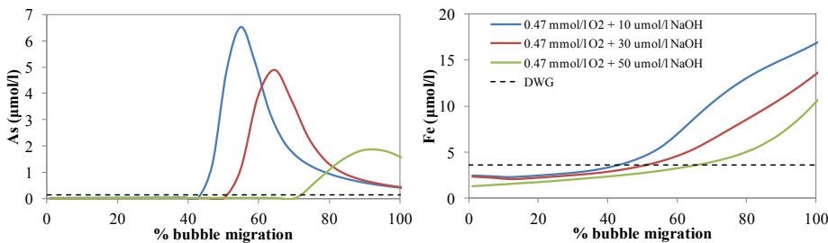
Figure 4.10. Evolution of As and Fe(II) concentrations in the ASR well during a complete bubble migration after having created a 100% efficient buffer zone with urban storm water and O 2 / NaOH addition. DWG = Drinking Water Guideline.
