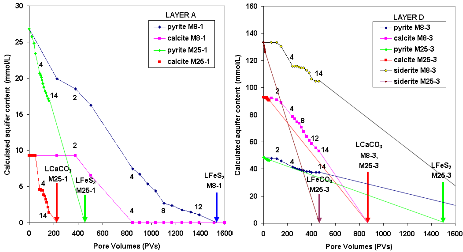
Figure 2.11 Calculated leaching of aquifer layer A (left; no siderite present) and D (right) during ASR cycles 1-14 and thereafter. Calculated is the average mineral content between the ASR well and the observation well. LX = leach factor for X. Numbers within graph refer to cycle number.
