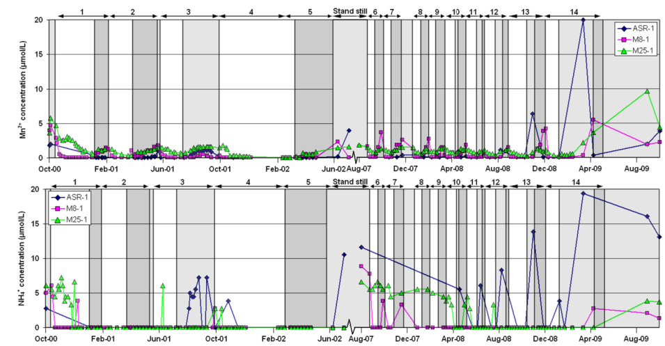
Figure 2.7 Plot of Mn and \text{NH}_4 concentrations in layer A over time, showing an anomalous Mn and \text{NH}_4 mobilization only in monitor well ASR-1 within the ASR proximal zone. 1-14 = cycle numbers; colored bands: white = injection, light grey = storage, dark grey = recovery.
