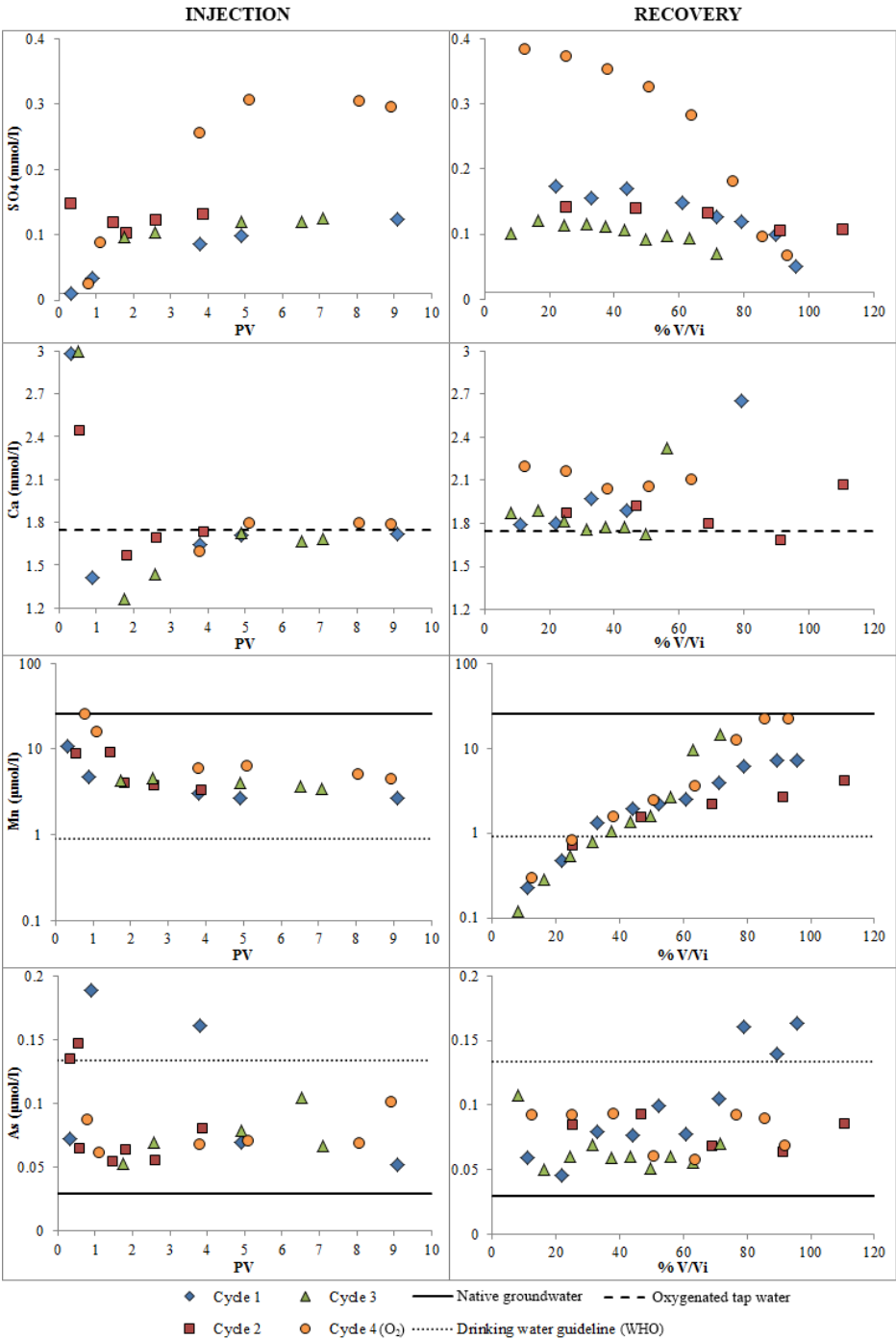
Figure 5.3. Water quality changes during the 4-cycle conventional ASR operation (experiment 1).
