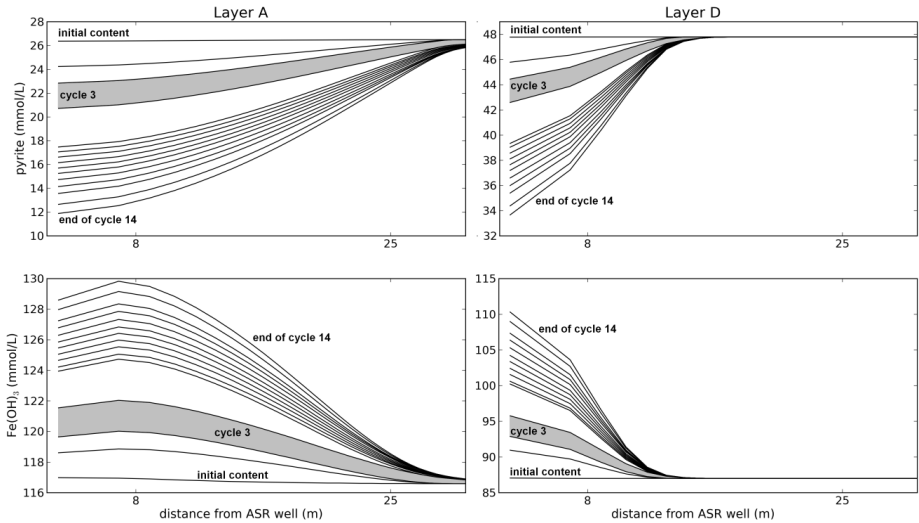
Figure 3.9 Pyrite content (above) and neo-formed Fe-hydroxide precipitates (below) versus distance at the end of each cycle. The positions of monitoring wells M8 and M25 are marked on the X axis.
